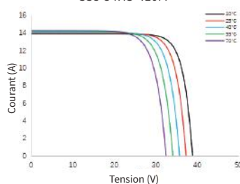
Courbe courant - tension SS8-54HS-410M
