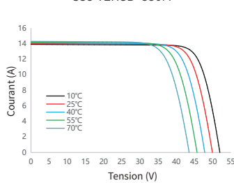
Courbe courant - tension SS8-72HSB -550M
