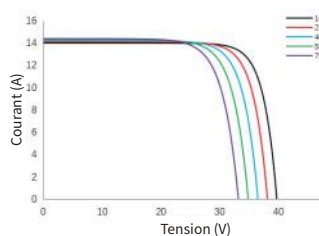
Courbe courant - tension SS8-54HDB-420N
