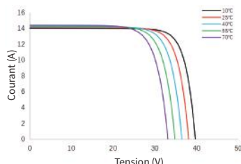
Courbe courant - tension SSA-48HD-445N
